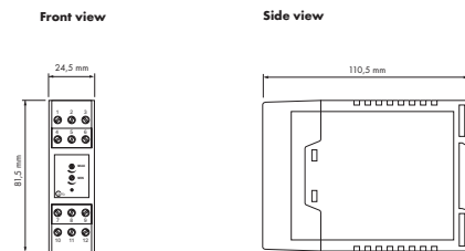
Installation to DIN rail of 35 mm wi
